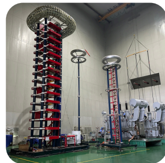
High-Voltage Testing Tower
